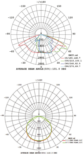
INTENSITY DISTRIBUTION DIAGRAM IN C PLANS
