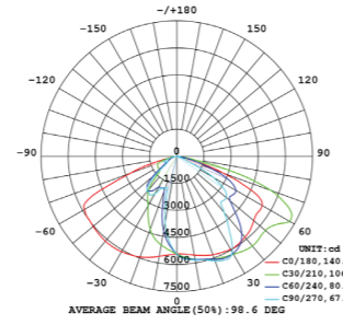
INTENSITY DISTRIBUTION DIAGRAM IN C PLANS
