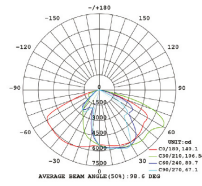
INTENSITY DISTRIBUTION DIAGRAM IN C PLANE
