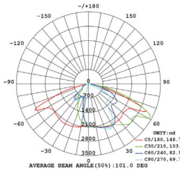
INTENSITY DISTRIBUTION DIAGRAM IN C PLANS
